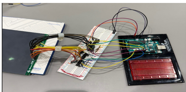
Figure 3: Connected Arduino, Circuit, and FSR
