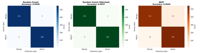
Figure 5: Model Confusion Matrices (Thursday)
