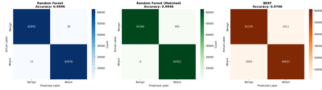
Figure 4: Model Confusion Matrices (Wednesday)
